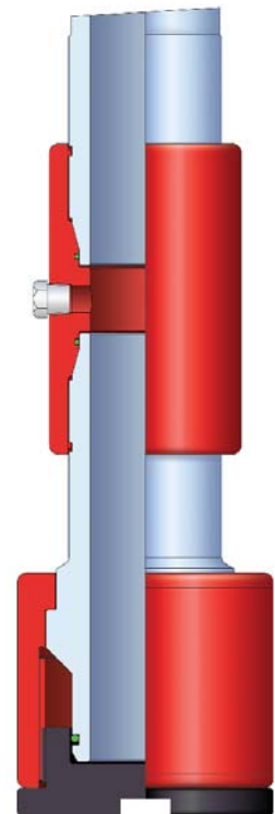
Conventional Lubricator
